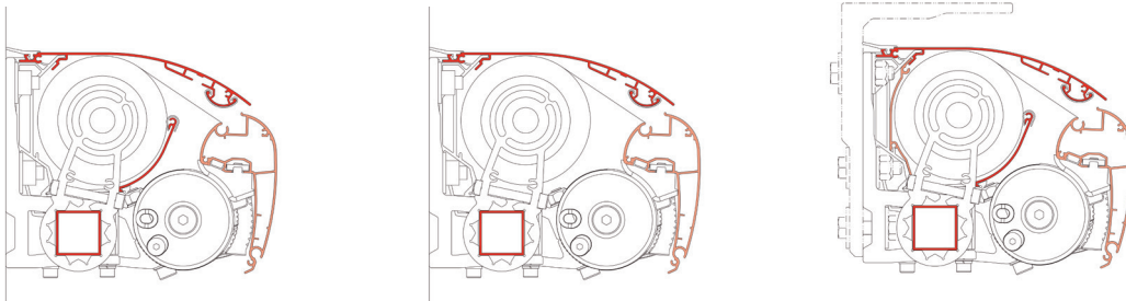
Installation frontale
