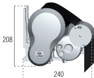
Installation frontale
