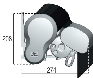
Installation frontale
